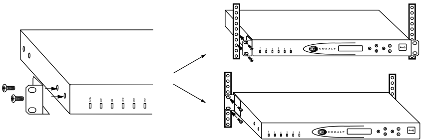
Figure 7. Mounting ears for the RaQ 4
