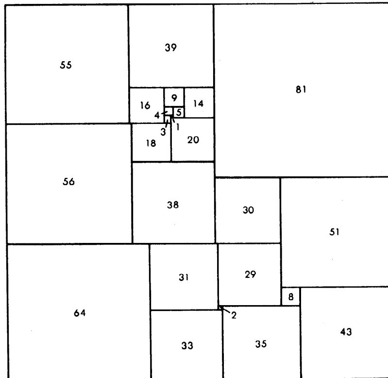
Figure 3(a). The smallest known (in 1961, and yet today as far as we know) squared square. Reprinted by special permission from Martin Gardner, The Second Scientific American Book of Mathematical Puzzles and Diversions , 1961, Simon and Schuster, New York, New York.
