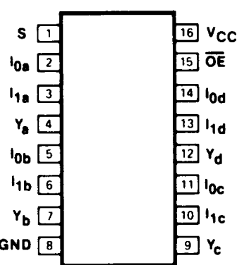
PIN ASSIGNMENT
