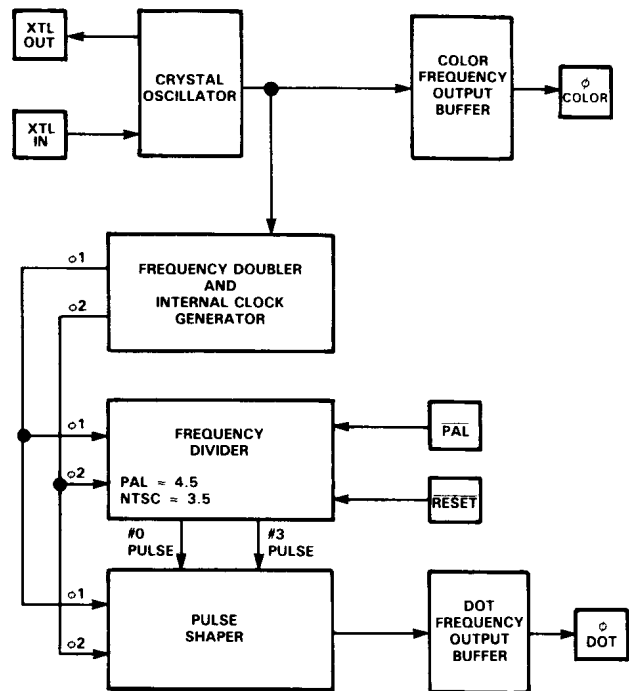
Block Diagram
