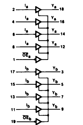
LOGIC DIAGRAM
