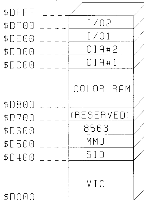
I/O Block
