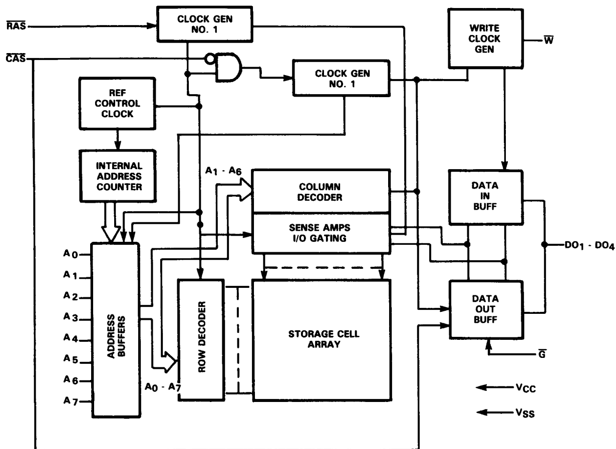
Functional Diagram
