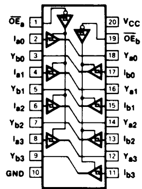
PIN ASSIGNMENT
