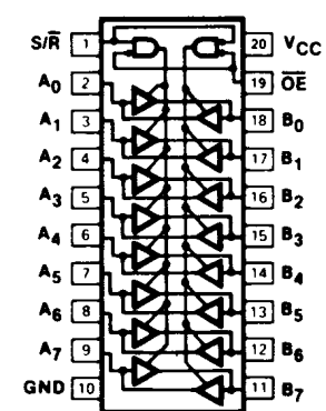
PIN ASSIGNMENT
