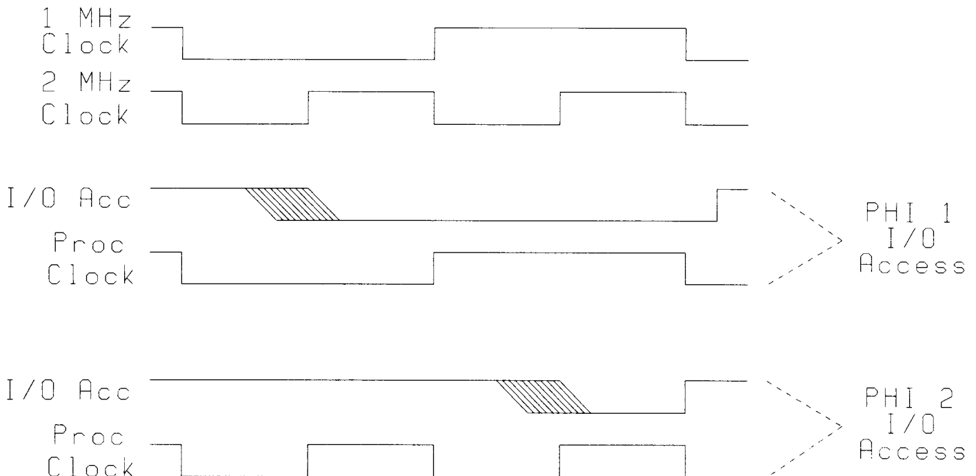
Clock Stretching in 2 MHz Mode
