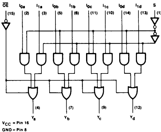
LOGIC DIAGRAM
