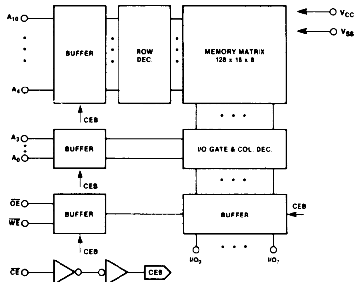
Functional Diagram
