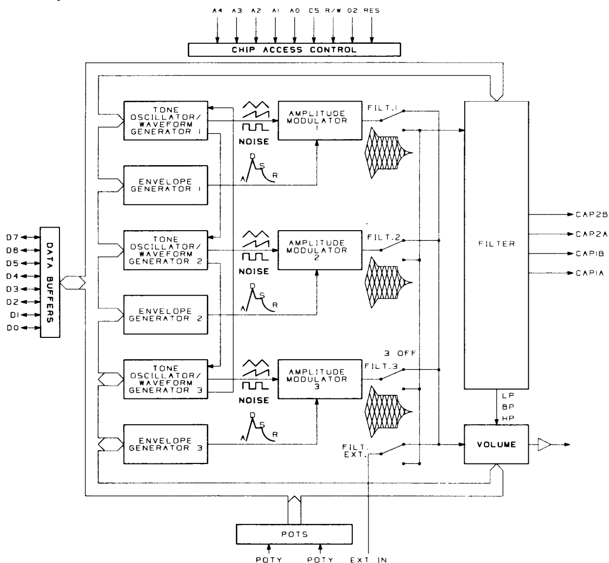
SID BLOCK DIAGRAM
