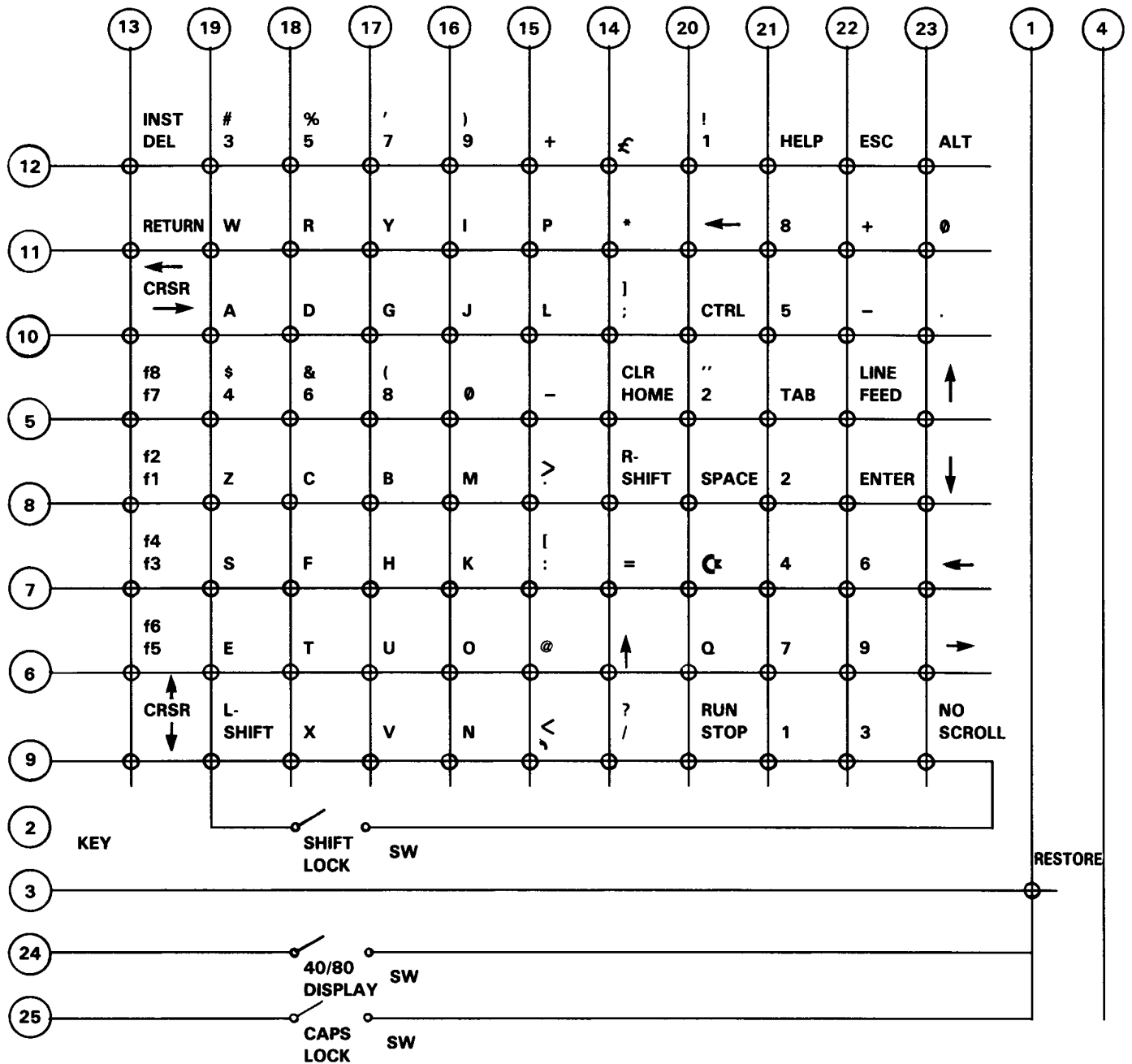
KEYBOARD MATRIX
