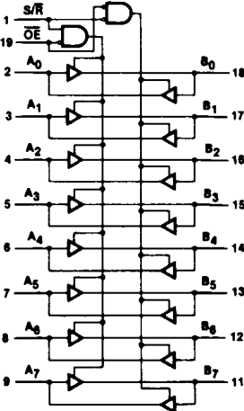
LOGIC DIAGRAM
