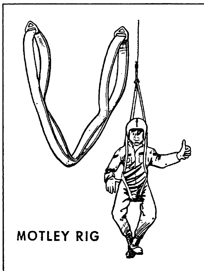
Figure 2-22. Motley rig
