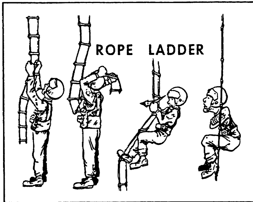
Figure 2-26. Rope ladder
