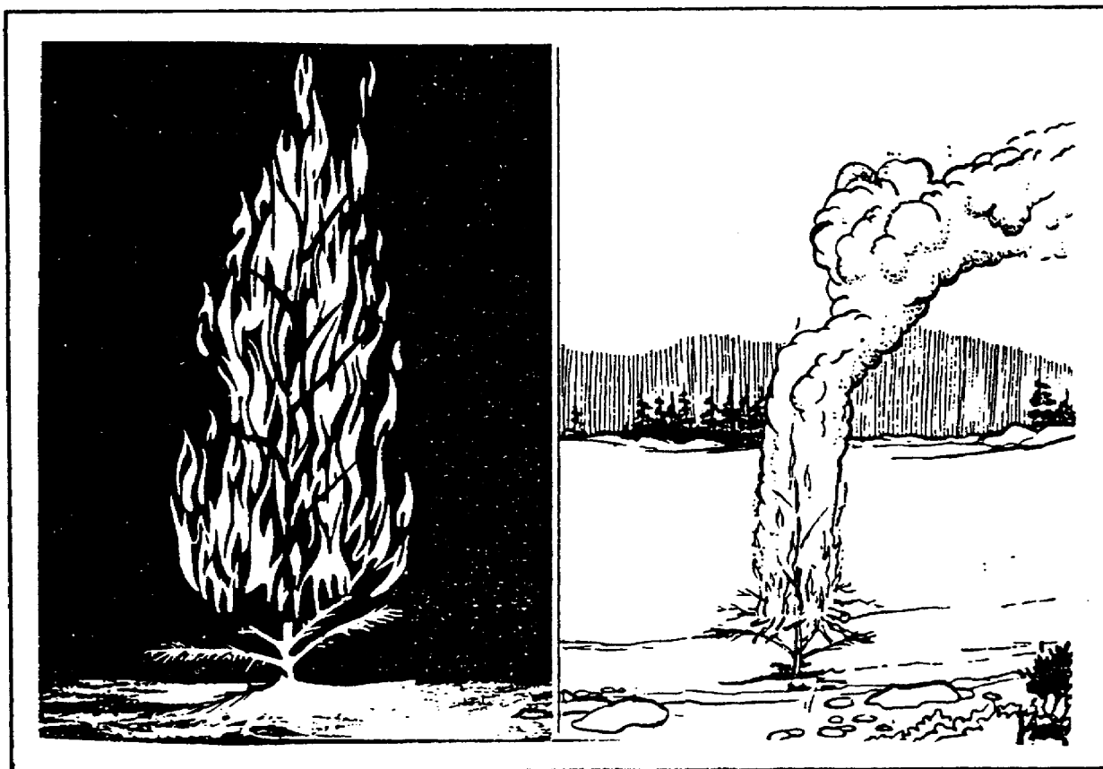
Figure 2-13. Tree torch
