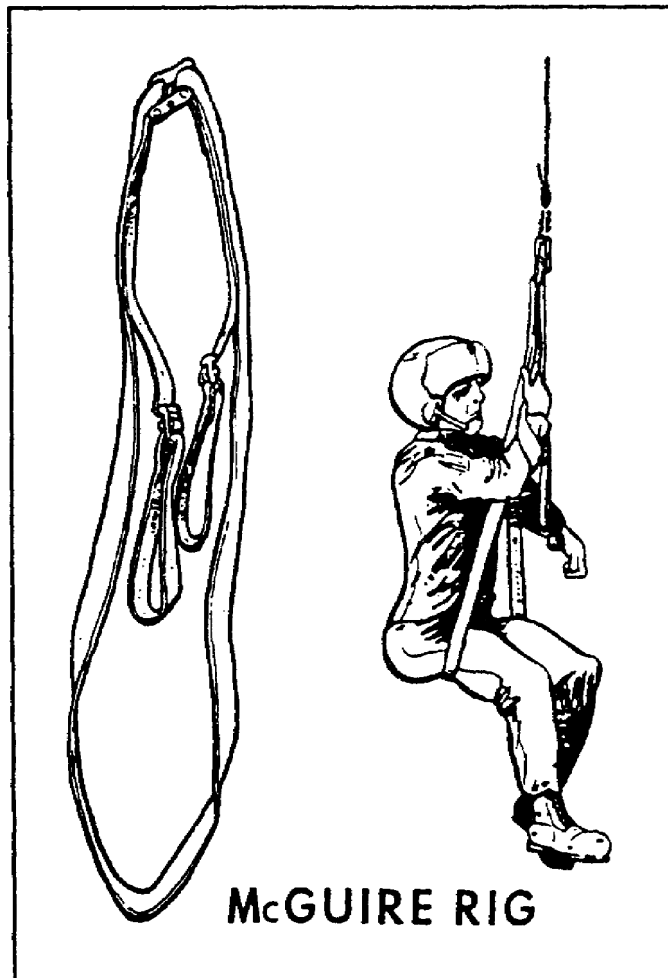
Figure 2-23. McGuire rig
