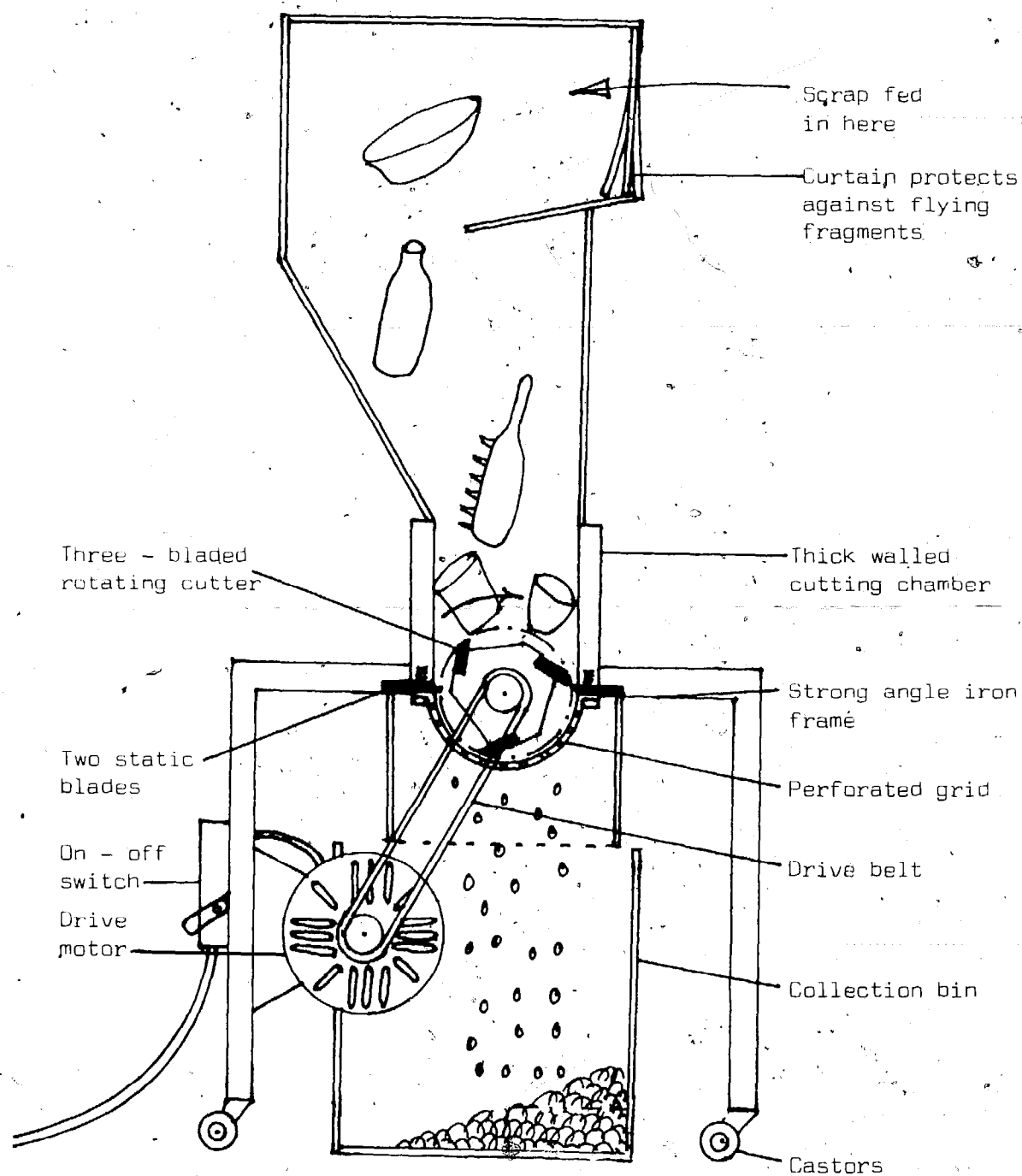
FIGURE 16: Granulator - (horizontal axis).
