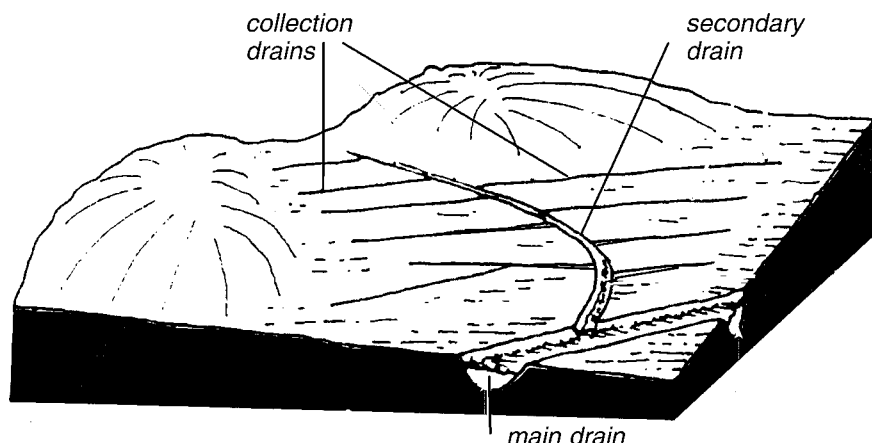
Figure 29: Drainage system
