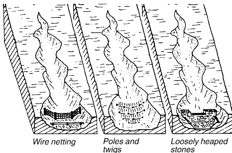
Figure 31: Controlling smaller gullies: view from above
