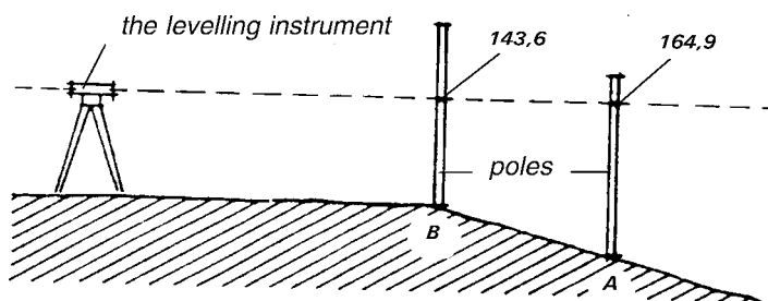
Figure 34: Height measurements with levelling instrument
