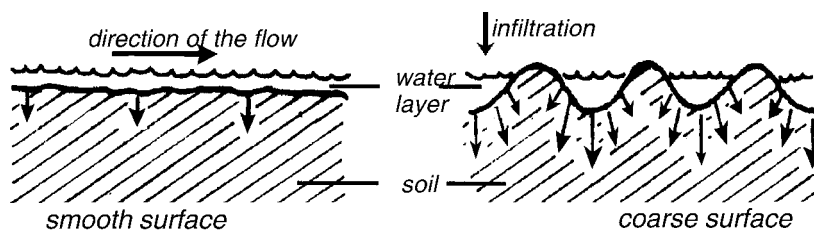
Figure 11: Run off on smooth surface and infiltration in coarse surface
