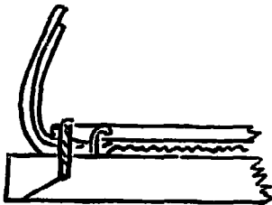
Type 3. Tack-lasted, machine-sewn sole
