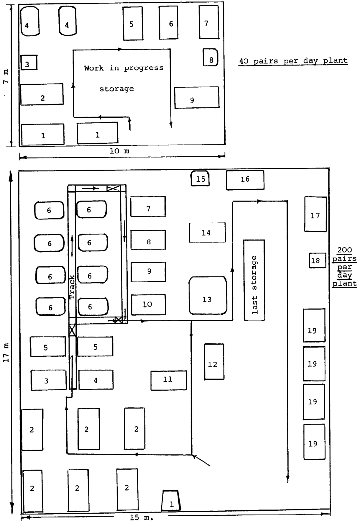
Figure II.14 Layout of production areas for type 1 footwear - 40 and 200 pairs per day
