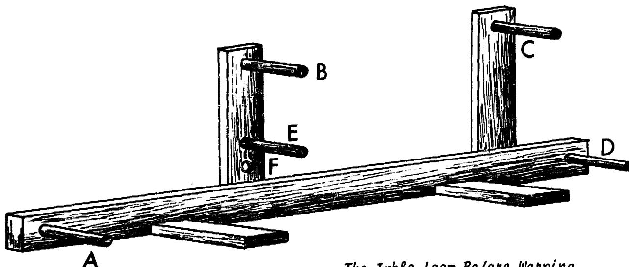
The Inkle Loom Before Warping
