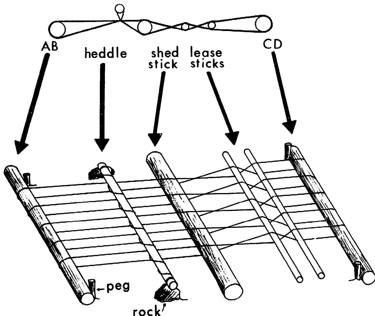
Side View (above) and Schematic view (below) - Peg Loom - showing working parts in position and pegs in place.
