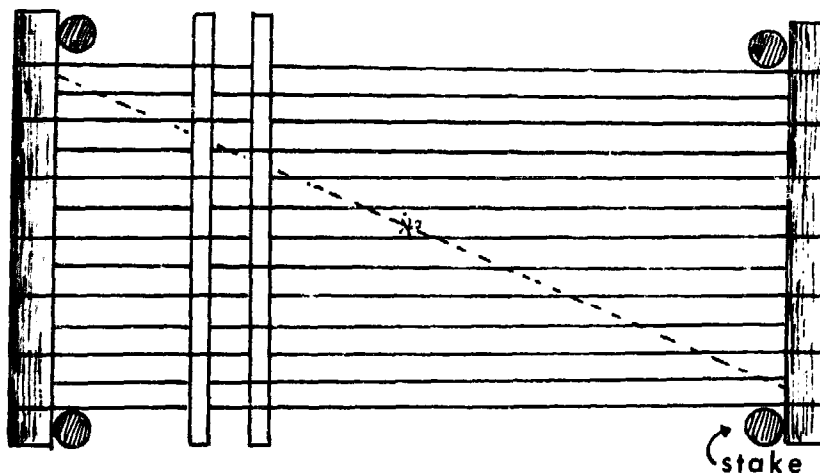
Step 5 - Warped crosspieces lying flat on ground showing beginning warp tied to the end warp.
