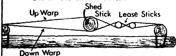
Side view without heddle
