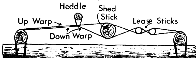
Side view with heddle in place
