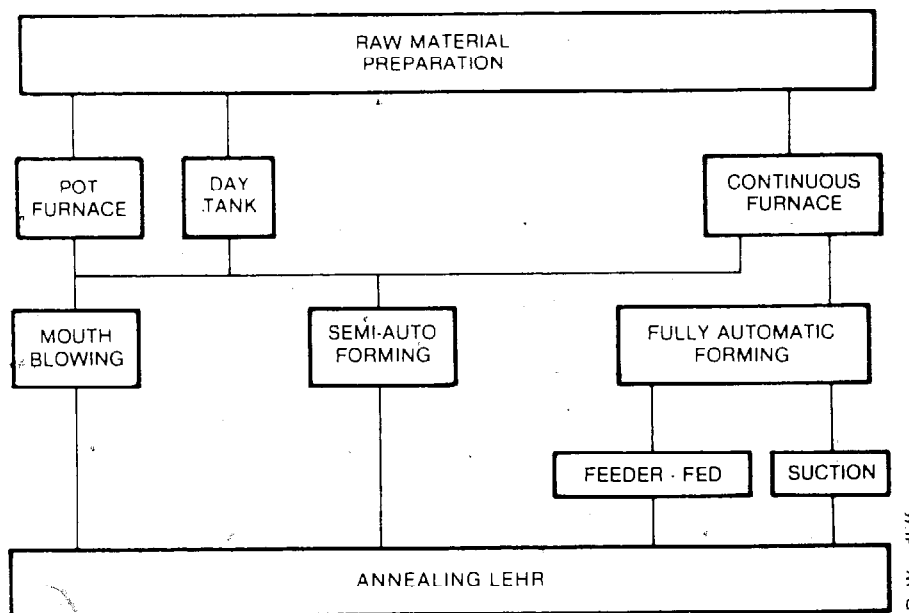
Figure 2: A diagrammatic representation of the processes involved in glass manufacture.
