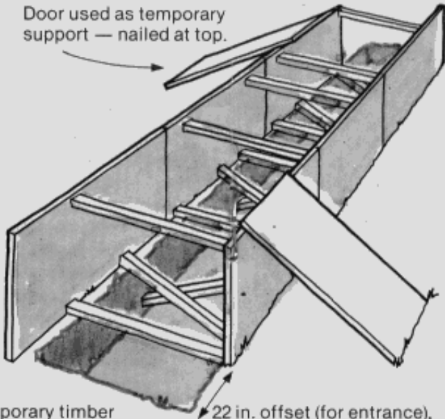
Fig 6 Construct temporary walls
