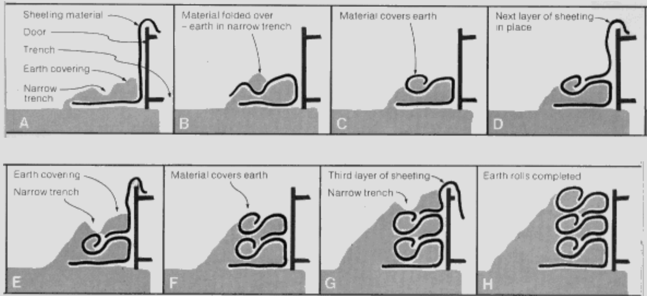
Fig 8 - Construction of earth rolls
