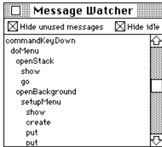
Figure 3-9 The Message Watcher window
