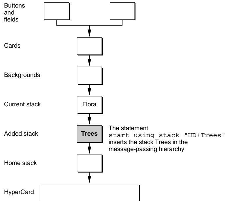
Figure 4-7 One stack added to the message-passing hierarchy
