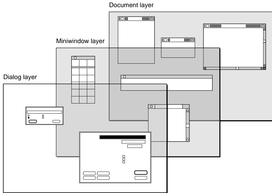
Figure A-2 HyperCard window layers
