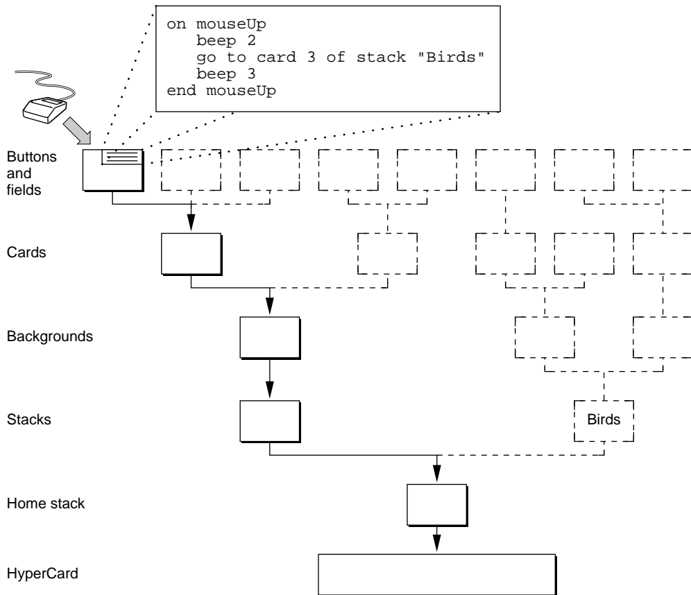
Figure 4-10 Static path before the go command executes
