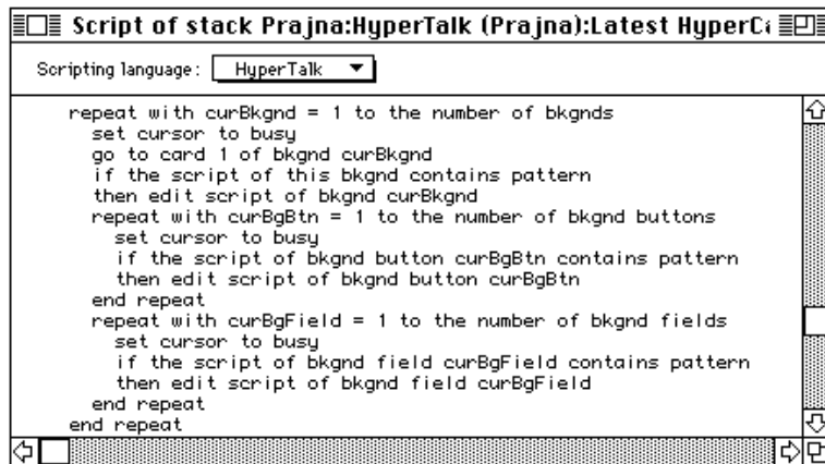
Figure 3-7 Nested control structures
