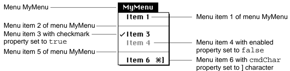
Figure 5-5 A custom menu
