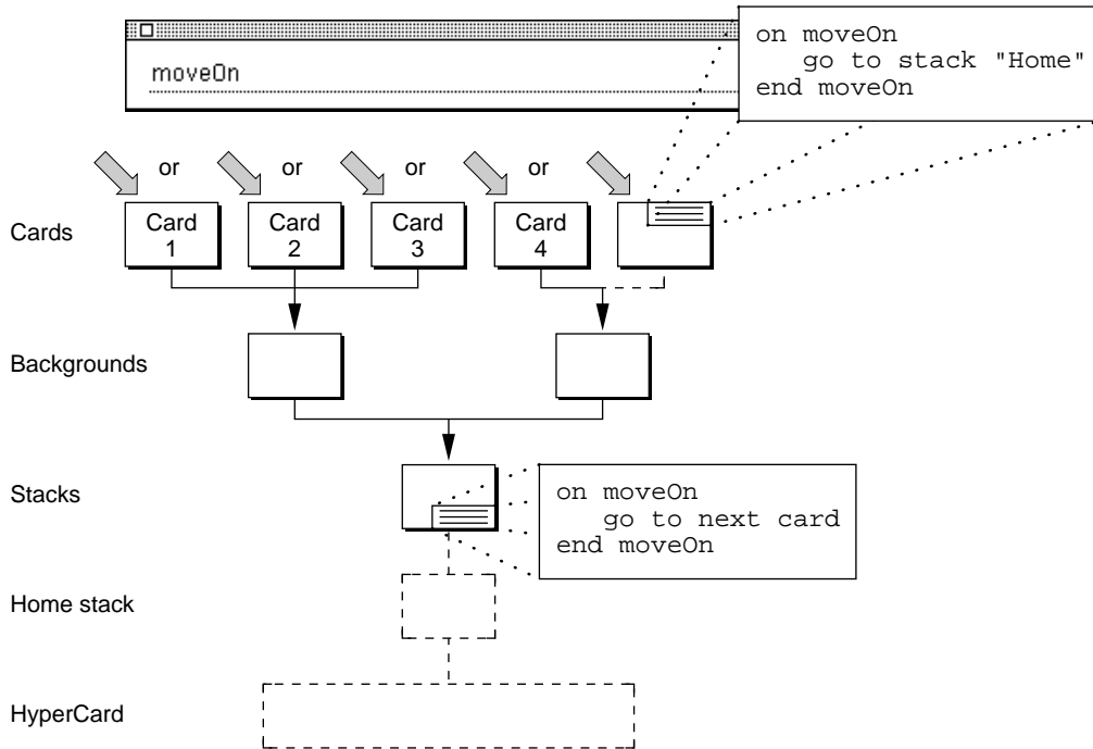
Figure 4-15 Intercepting a message
