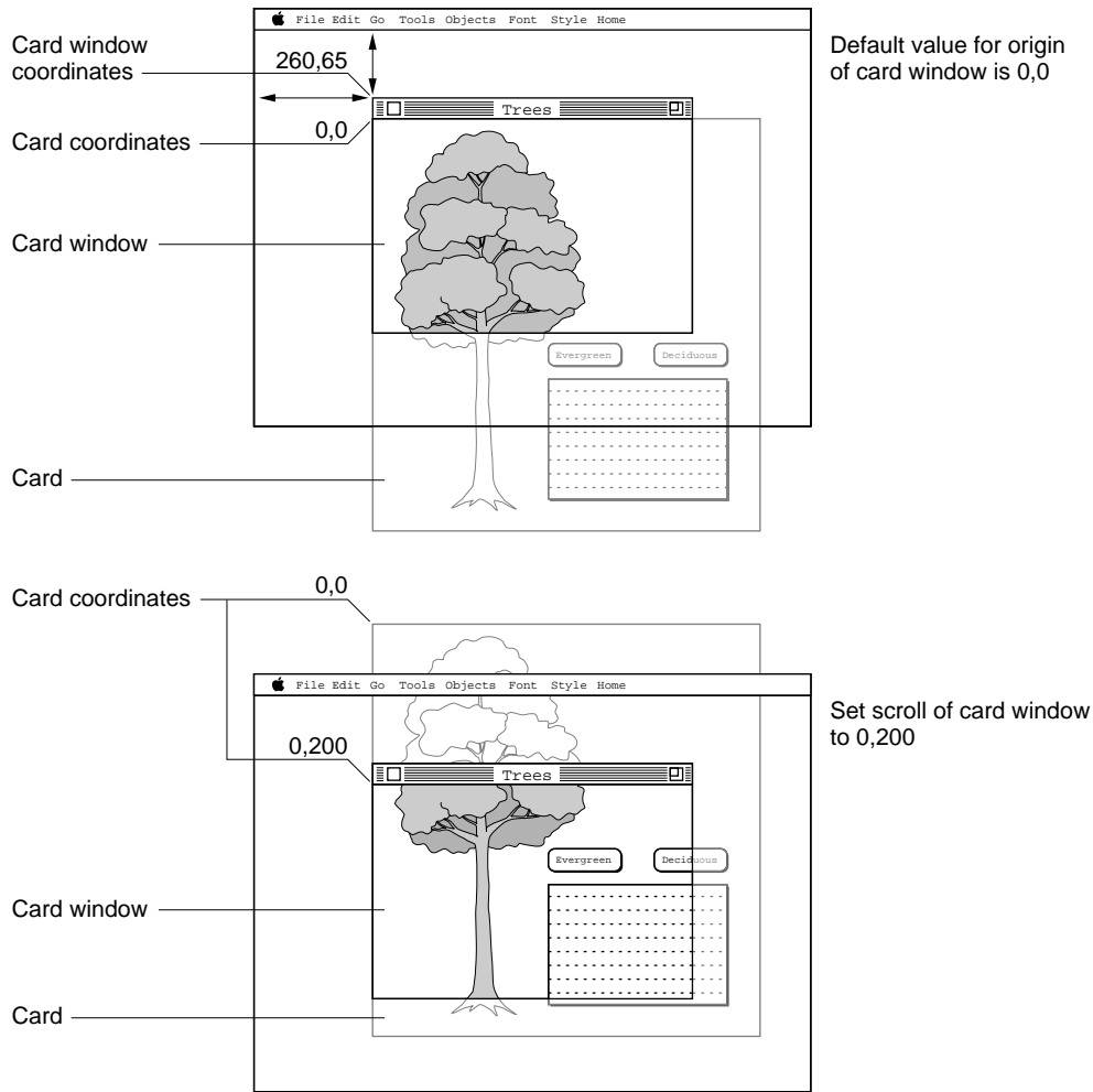
Figure 2-2 Relationship between the location of a card and a card window
