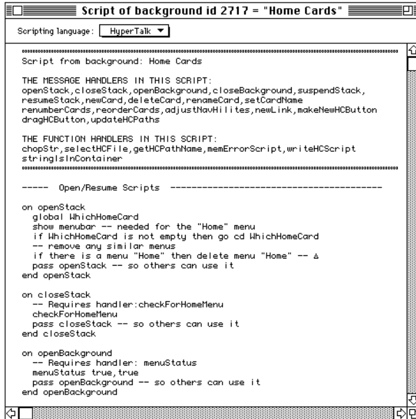
Figure 3-3 Script editor window
