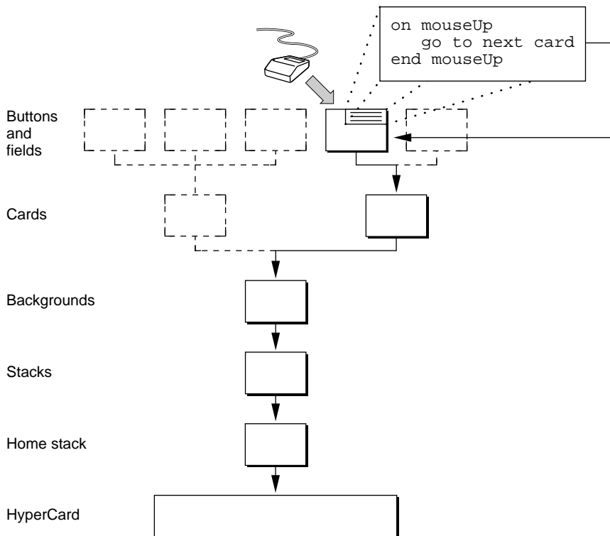
Figure 4-5 Command sent as a message
