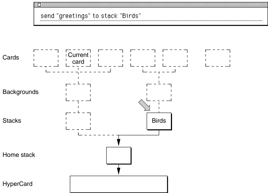
Figure 4-12 Using the send keyword
