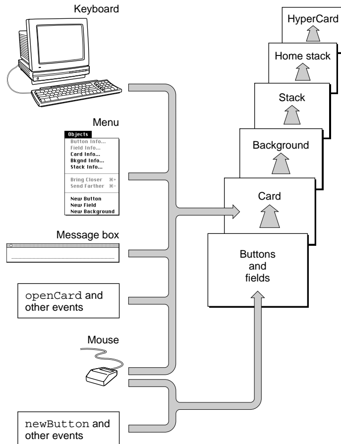
Figure 4-2 Message-passing hierarchy
