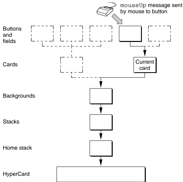
Figure 4-4 Message traversing current hierarchy
