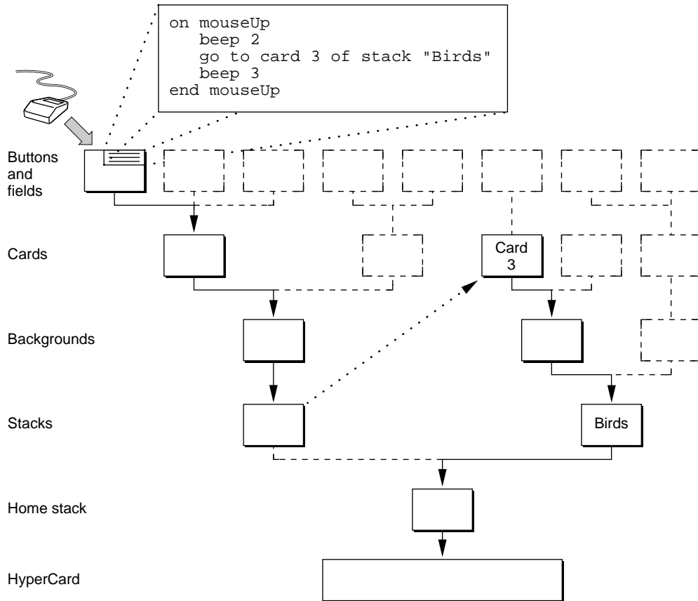
Figure 4-11 Dynamic path after the go command executes
