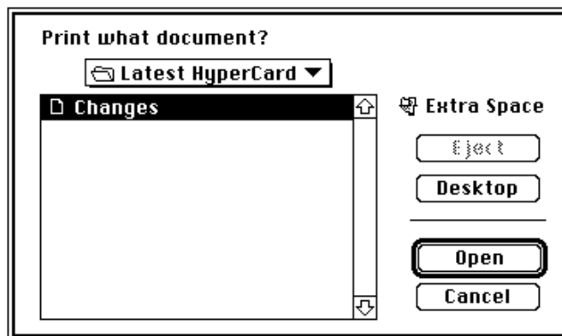
Figure 10-2 Answer command display of the standard file dialog box
