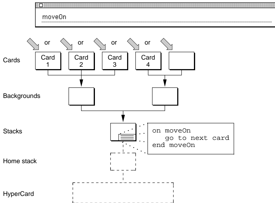
Figure 4-14 Handler in a stack script
