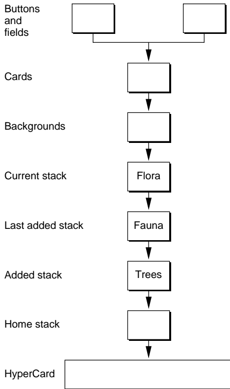
Figure 4-8 Two stacks added to the message-passing hierarchy
