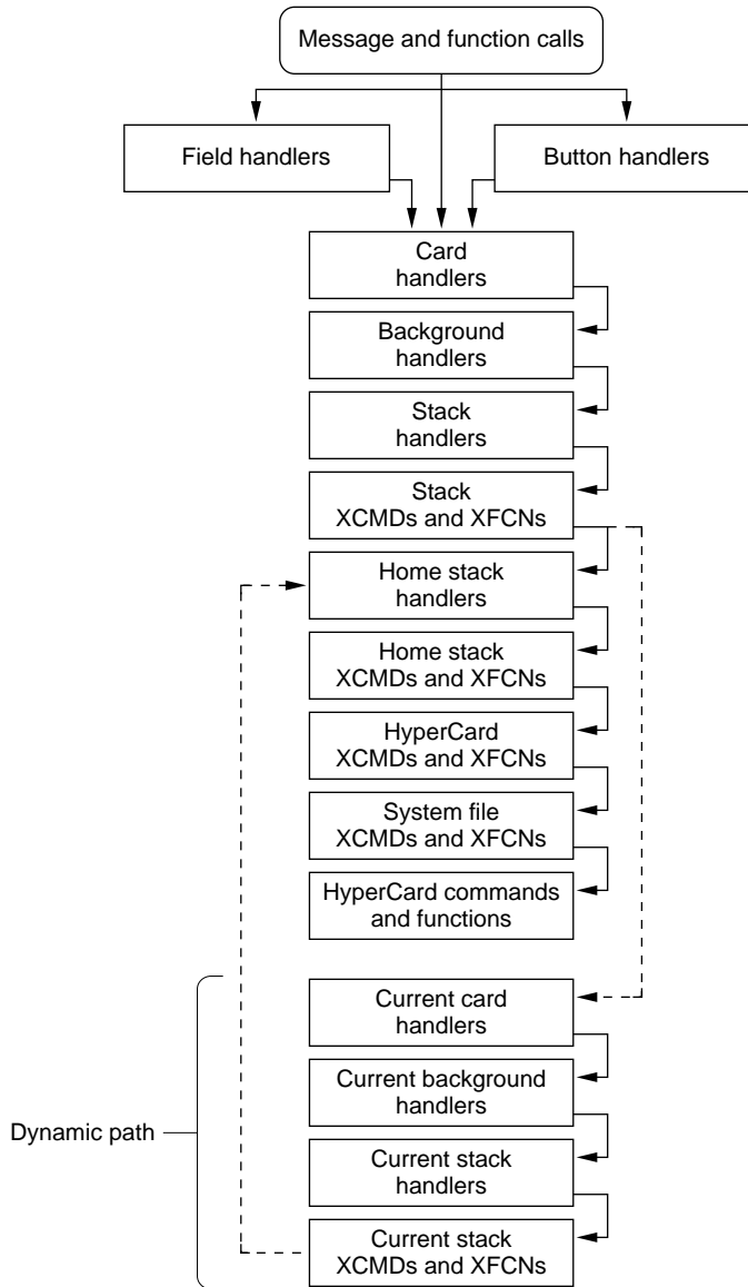
Figure A-1 Message-passing hierarchy, including XCMDs and XFCNs
