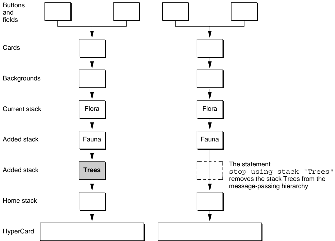
Figure 4-9 Removing a stack from the message-passing hierarchy
