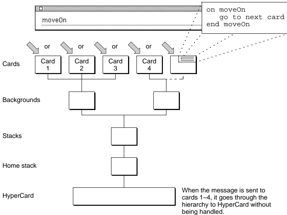
Figure 4-13 Handler in a card script
