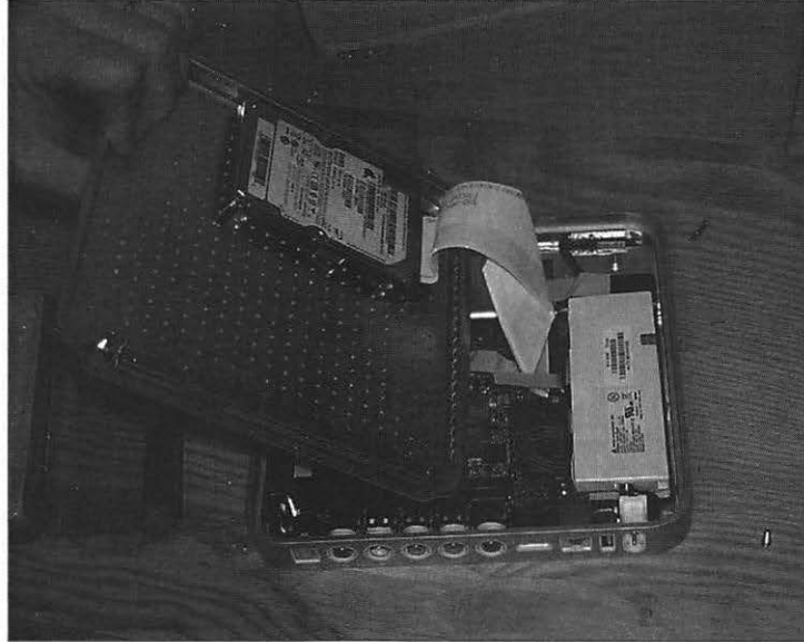
Figure 10-5. Gently opening the case
