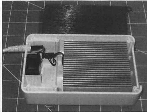
Figure 13-14. The aluminum heat sink exposed
