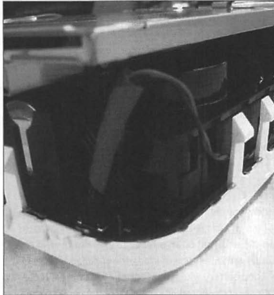
Figure 15-3. Extending the mini's power button
