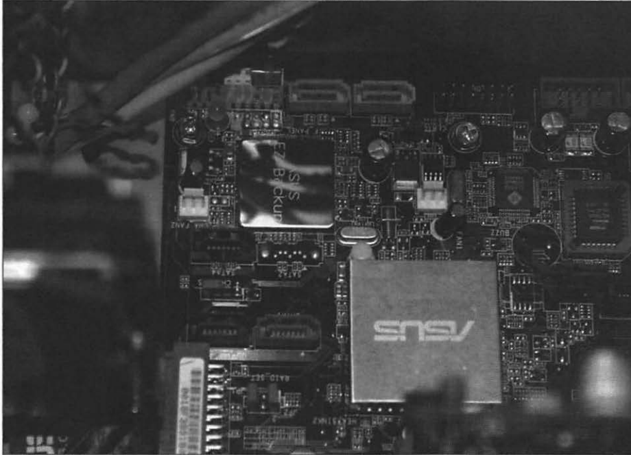
Figure 8-46. Most of the SATA connectors. Plug the hard drive into the RED one
