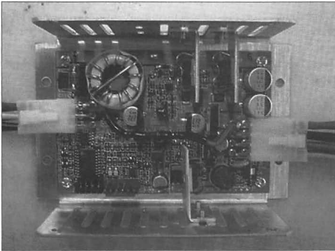
Figure 15-5. The Carnetix CNX-P1900
