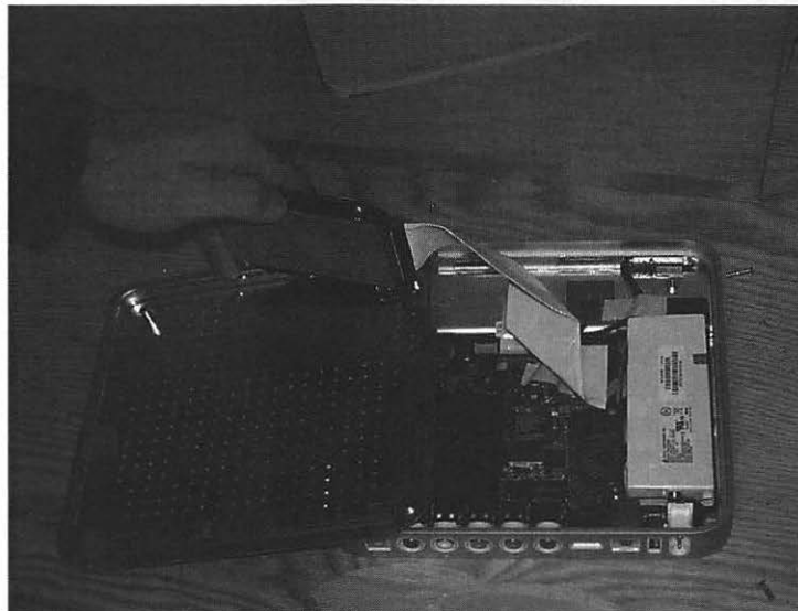
Figure 10-6. Removing the disk drive
