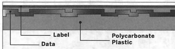
Figure 15-9. Idealized CD cross section
