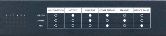
Figure 7 BPS-120 Front Panel DC Output LED Detail
