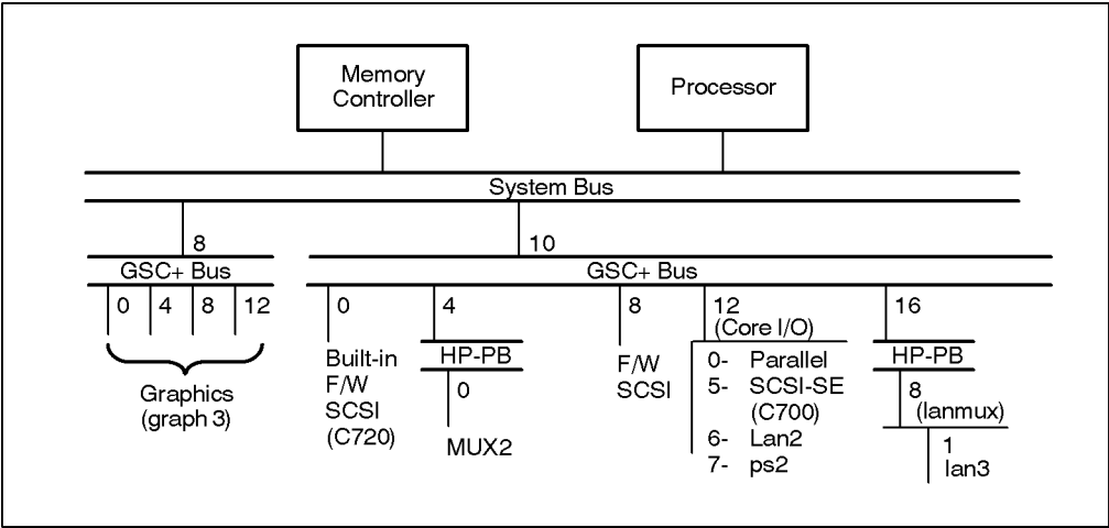
Figure B-8 Model 8x9 K Series Bus Relationships
