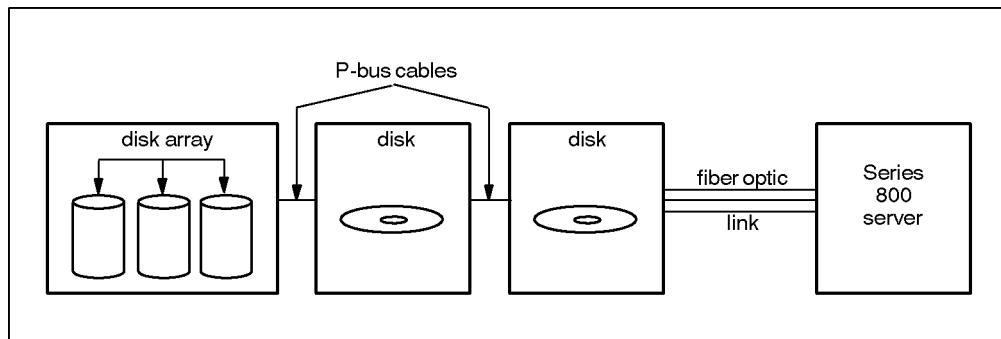
Figure 2-3 HP Fiber-Optic Connectivity
