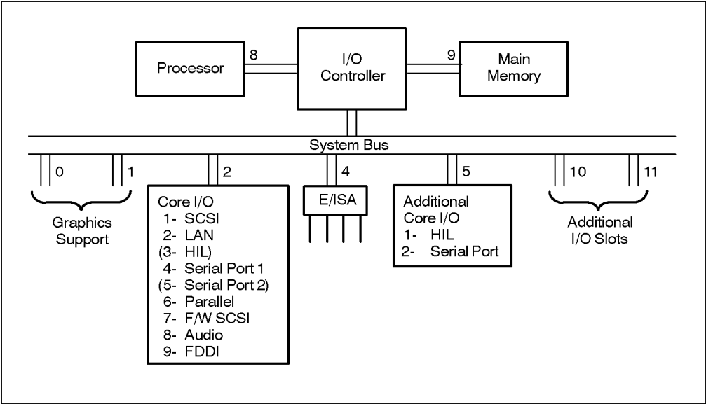
Figure B-2 Model 725/100 Bus Relationships
