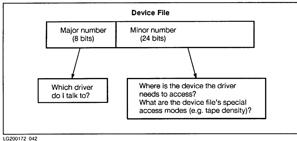
Figure C-1 Device Special Files Contain Major and Minor Numbers
