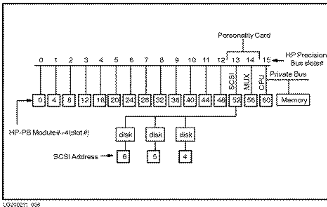
Figure B-6 Basic Addressing on Models F/G/H/I and 8x7 Systems
