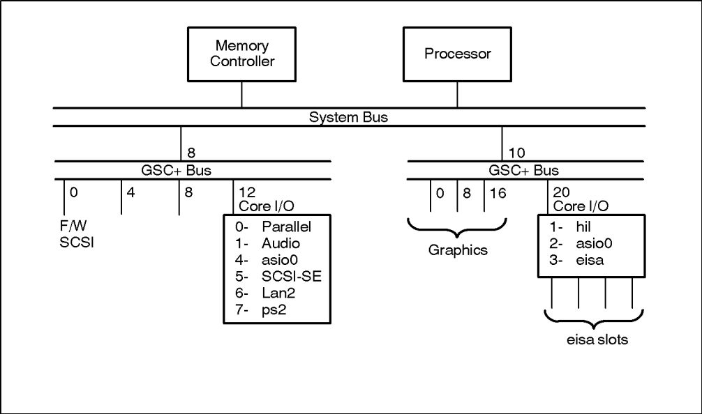
Figure B-3 Model 770 J Series Bus Relationships
