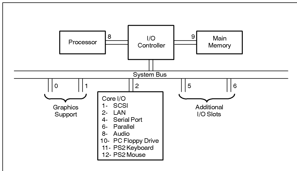
Figure B-1 Model 712 Bus Relationships
