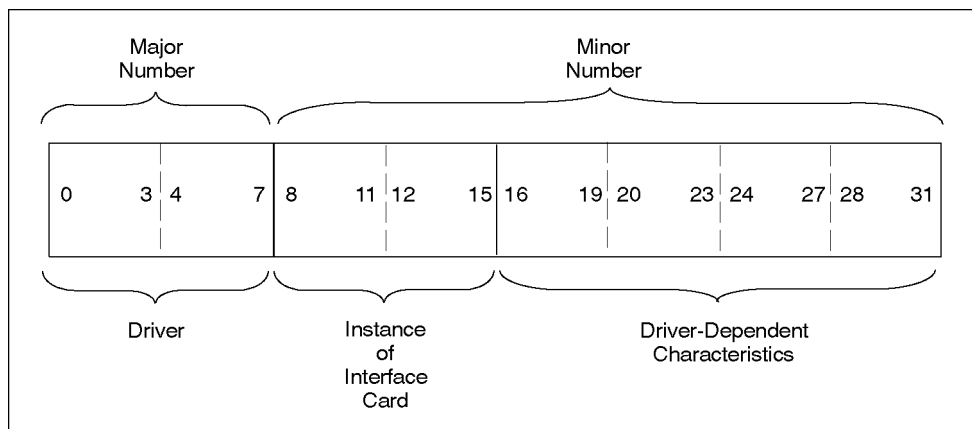
Figure C-2 Driver Number ( dev_t ) Format
