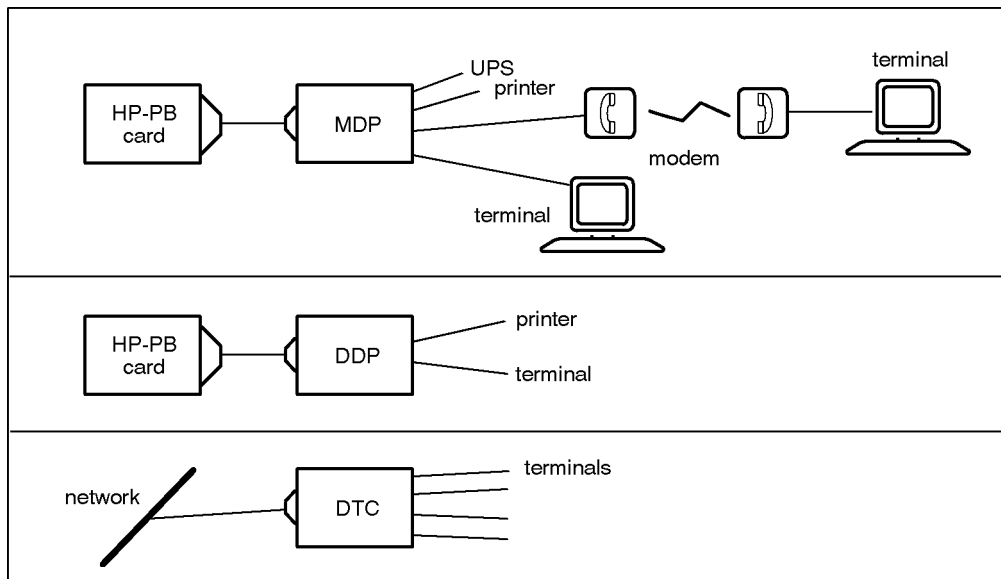
Figure 2-2 Serial Connectivity via Distribution Panels or DTC
