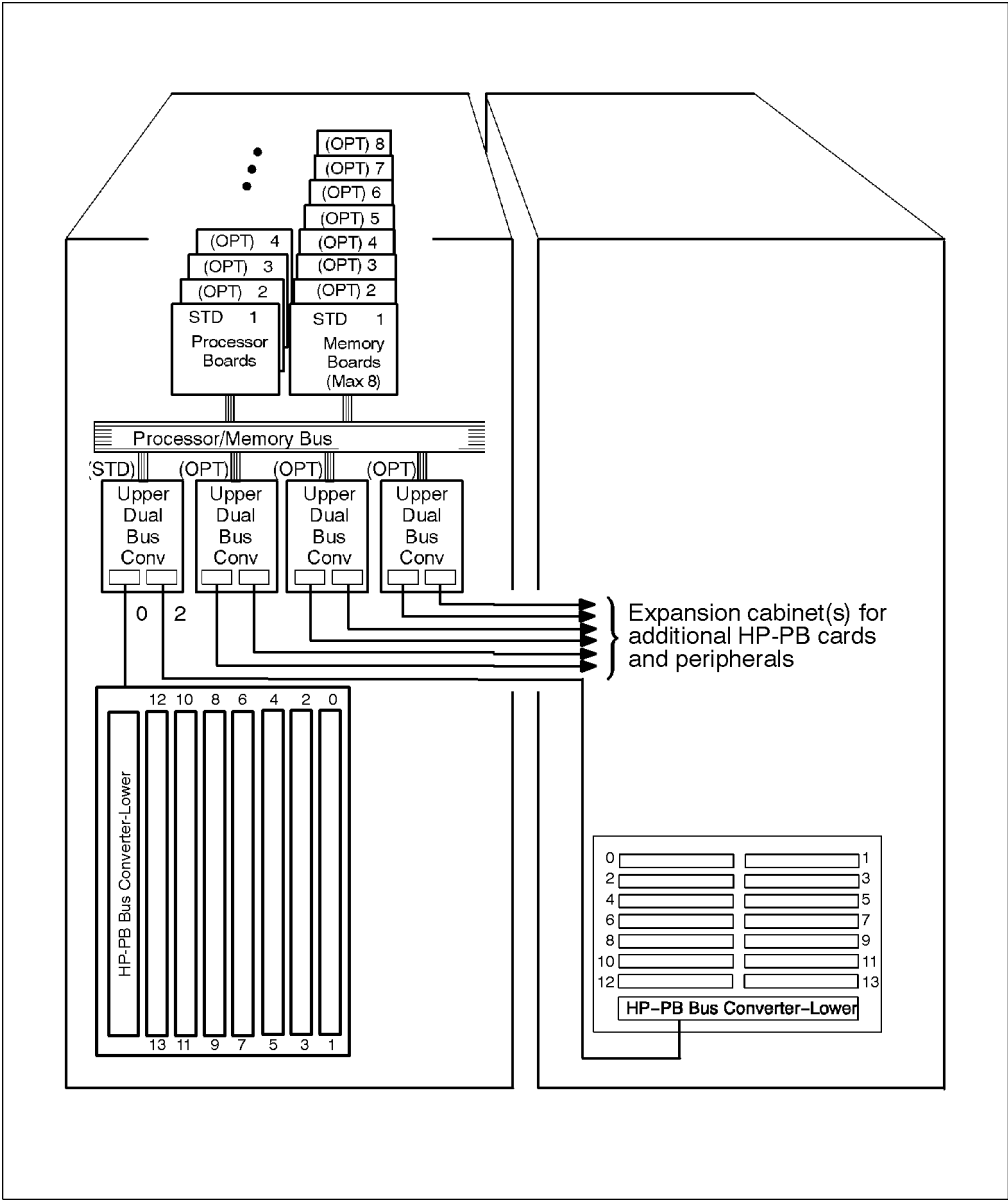
Figure B-7 HP 9000 T500 Configuration and Bus Relationships
