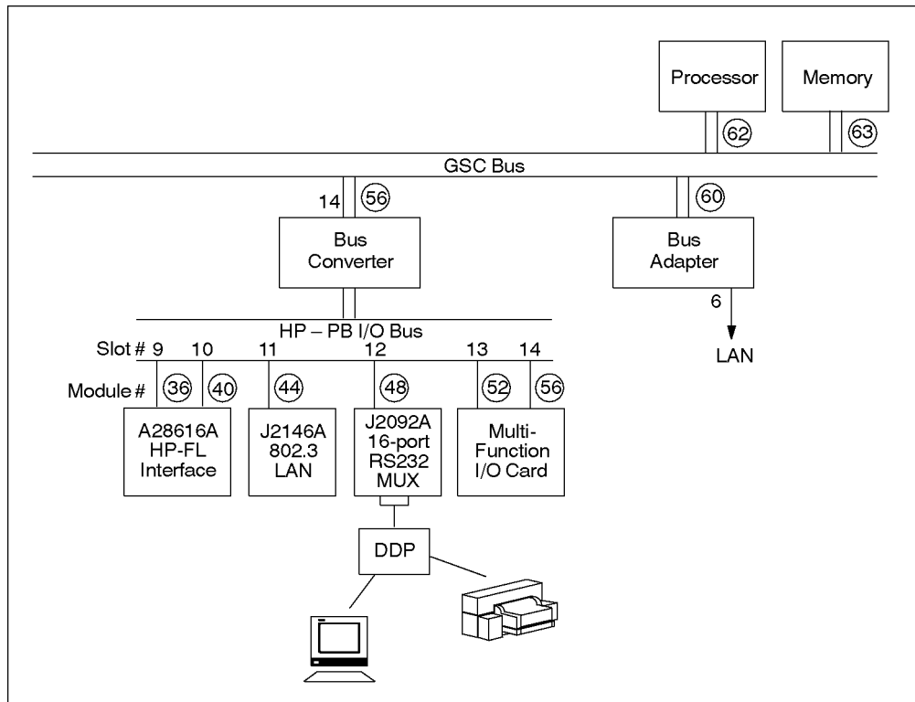
Figure B-4 HP 9000 Model E Bus Relationships
