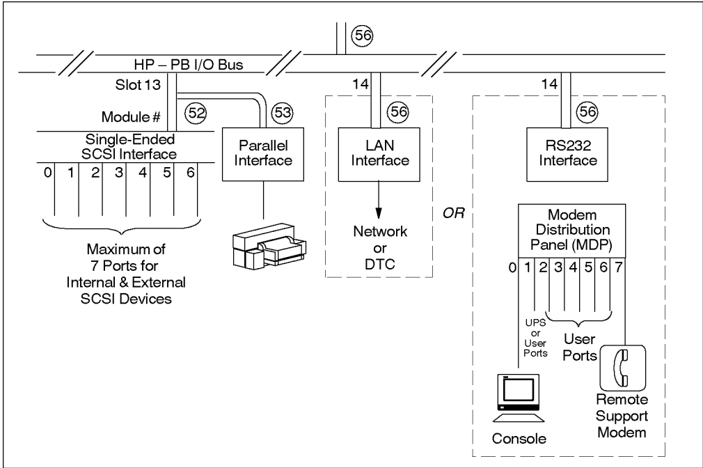
Figure B-5 Typical I/O Addressing for a MUX/SCSI Multi-Function Card
