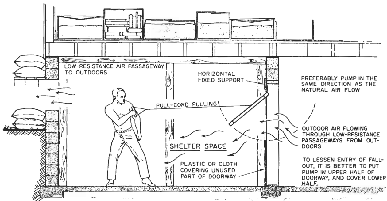
FIGURE 46: A KAP pictured in use in an improvised basement fallout shelter. The pump may also be operated comfortably from a
