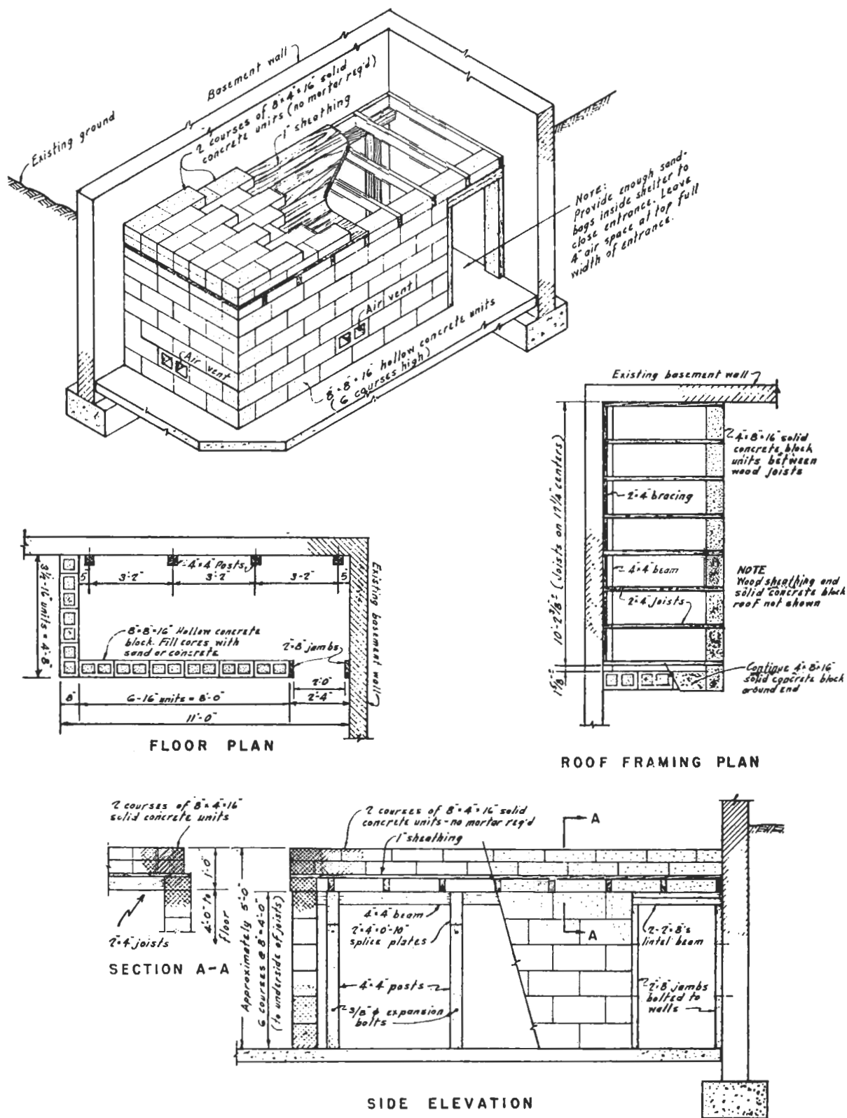
FIGURE 22: Prefabricated Basement Concrete Block Shelter. This type of shelter can be stored as components and then assembled quickly if necessary. In the building plans, note that the hollow blocks
