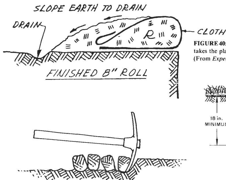
FIGURE 42: The proper way to use a pick or mattock. Work your way forward by breaking off chunks of the trench floor. Then shovel out the chunks. Don't try to do your primary digging with the shovel. (From Expedient Shelter Handbook .)
