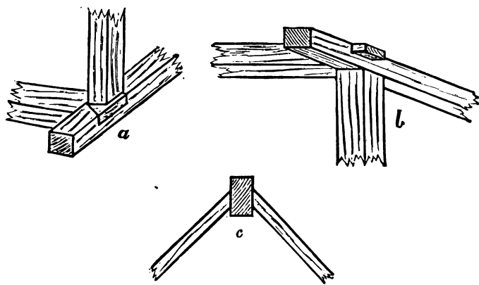
FIG. 57.—Joints employed in Out-house.
