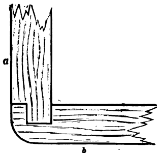
FIG. 68.—Tongued and grooved joint for small work.
