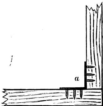
FIG. 52.—Spars joined by "angle" iron.
