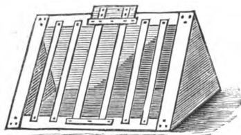
FIG. 61.—Hen-coop.
