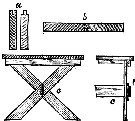
FIG. 51.—Summer-house Table.
