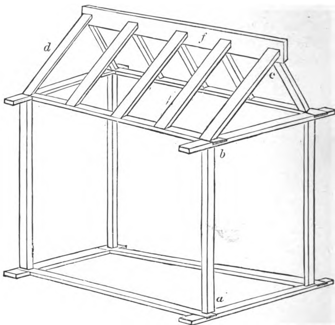
FIG. 56.—Frame-work of Out-house.
