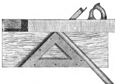
FIG. 91.—Shooting-board.
