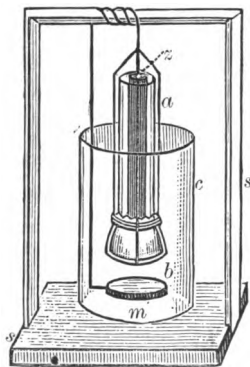
FIG. 139.—Simple arrangement for Electrotyping.
