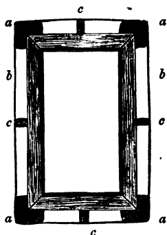
FIG. 92.—Blocks for Picture-frame fixing.
