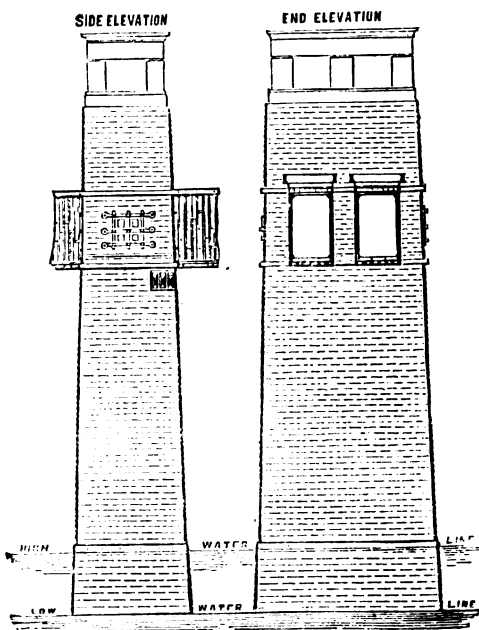
FIG. 98 a.—Land Tower.
