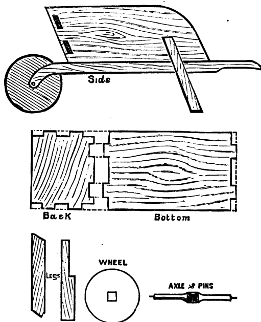
FIG. 69.—Wheelbarrow.
