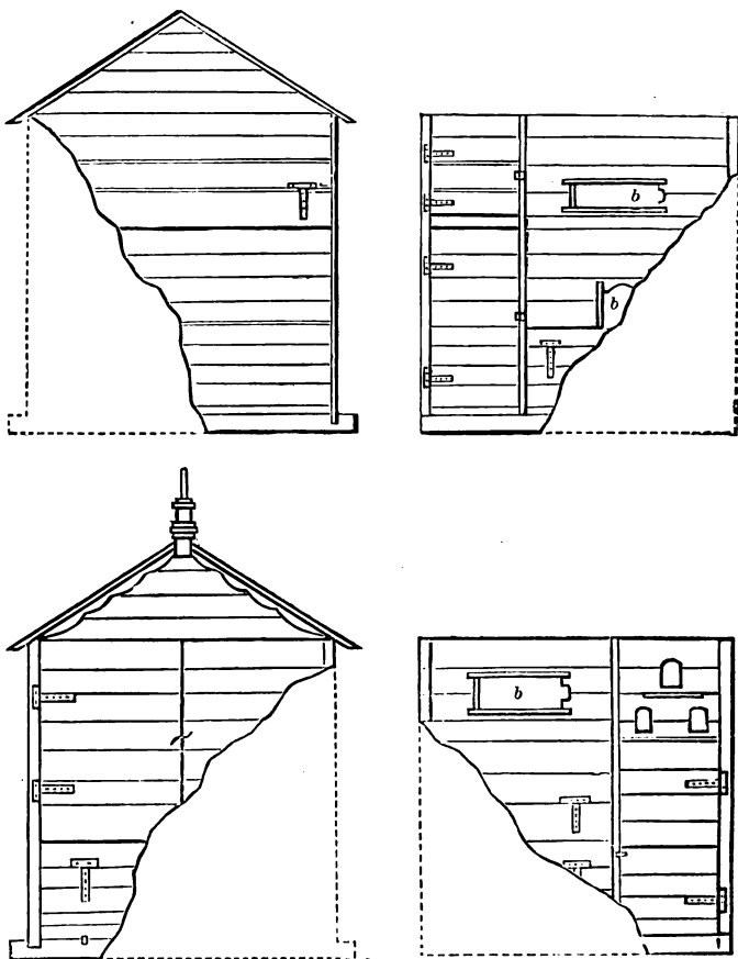
FIG. 58.—To show arrangement of Nest-boxes and Slip-doors.
