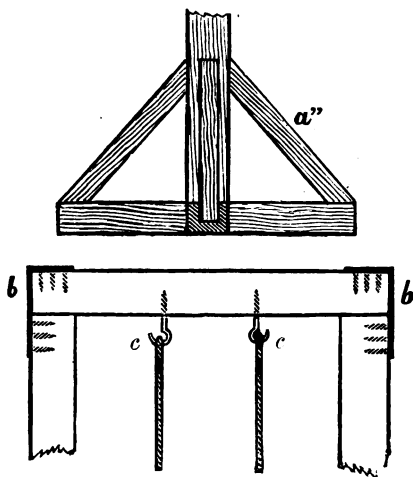
FIG. 47.—The Swing.
