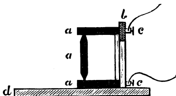
FIG. 150.—A Simple Microphone.
