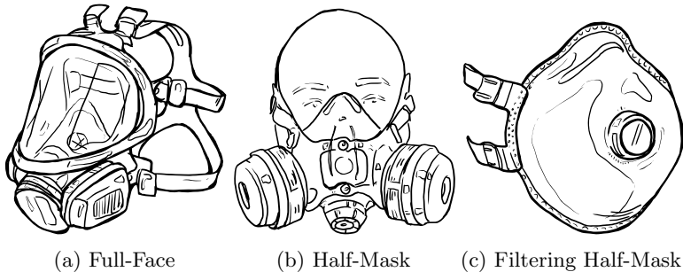
Figure 30.4: Types of Respirators 70
