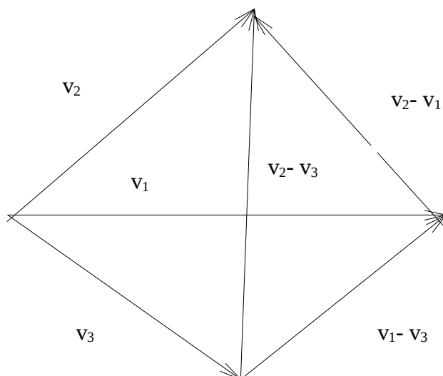
FIGURA 2: \Delta_1^2 + \Delta_2^2 = \Delta_3^2 + \Delta_4^2
