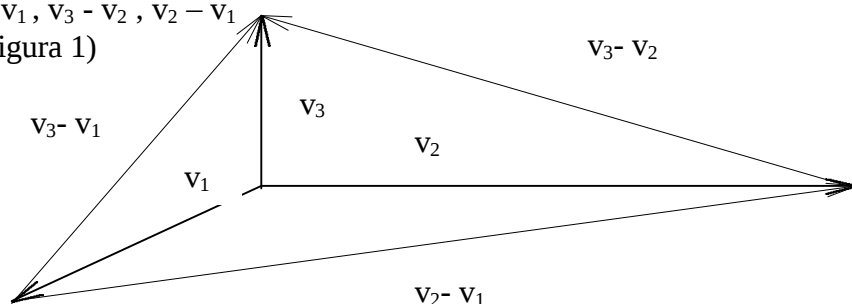
FIGURA 1: \Delta_1^2 + \Delta_2^2 + \Delta_3^2 = \Delta_4^2
