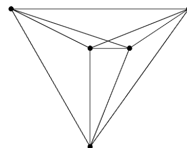
Figure 1 The complete graph with 5 nodes
