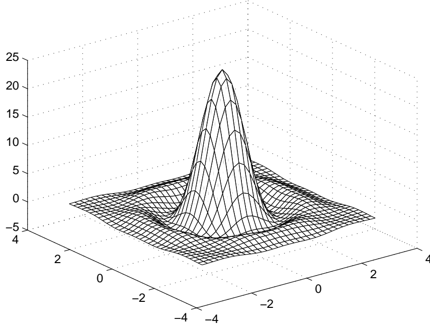
Figure 5.4: The Bochner-Riesz kernel K_n^{q,\alpha} with d = 2 , q = 2 , n = 4 , \alpha = 1 , \gamma = 2 .
