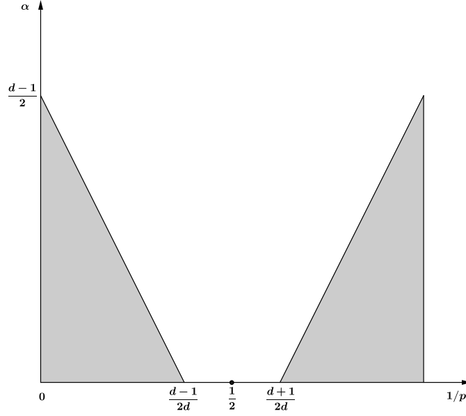
Figure 6.1: Uniform unboundedness of \sigma_n^{2,\alpha} .
