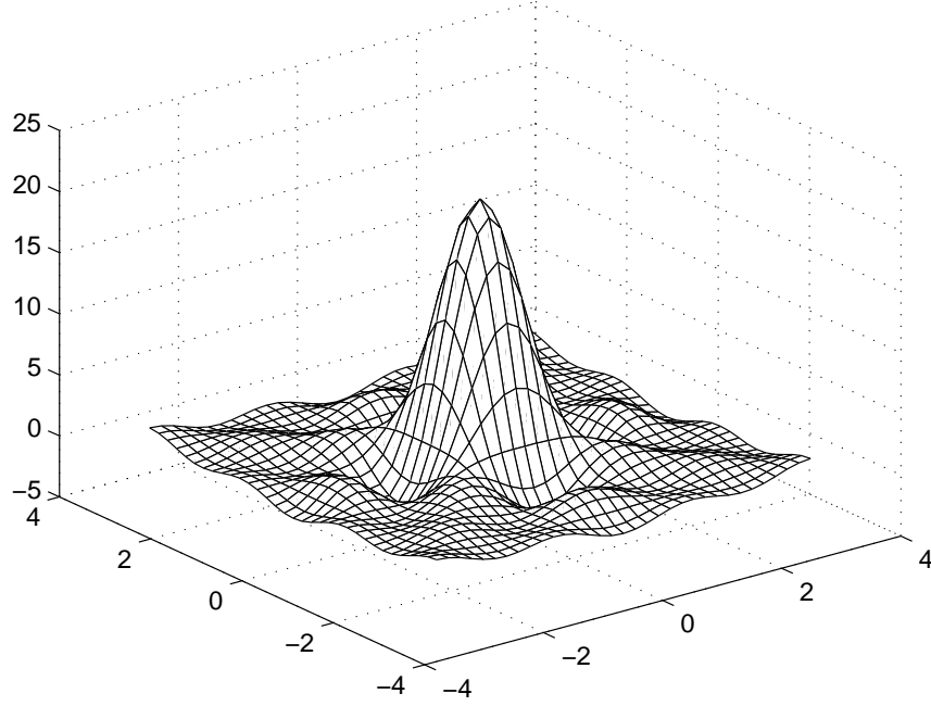
Figure 5.2: The Riesz kernel K_n^{q,\alpha} with d = 2 , q = \infty , n = 4 , \alpha = 1 , \gamma = 1 .
