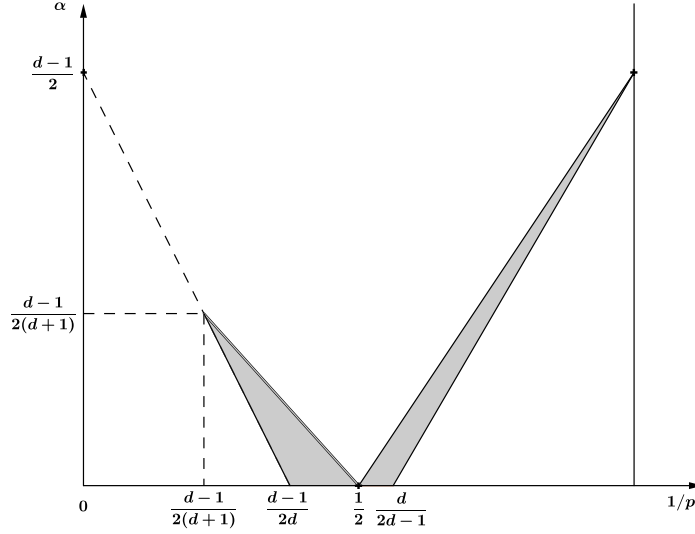
Figure 8.4: Open question of the boundedness of \sigma_*^{2,\alpha} when d \geq 3 .
