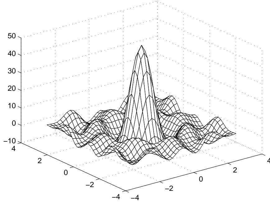
Figure 4.3: The Dirichlet kernel D_n^q with d = 2 , q = 2 , n = 4 .
