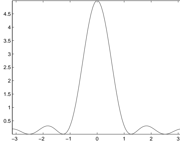
Figure 3.1: Fejér kernel K_n for n = 5 .
