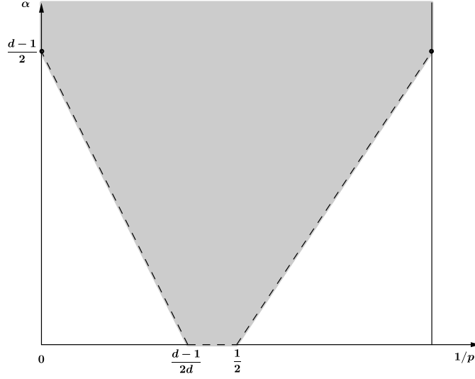
Figure 8.5: Almost everywhere convergence of \sigma_n^{q,\alpha} f , f \in L_p(\mathbb{T}^d) .
