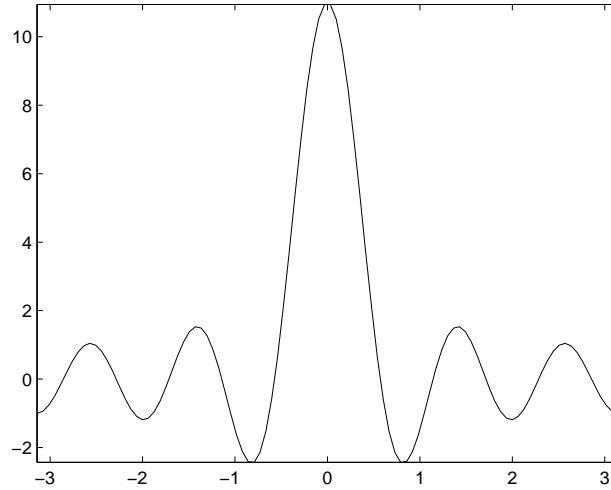
Figure 2.1: Dirichlet kernel D_n for n = 5 .
