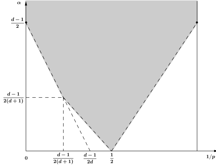
Figure 8.3: Boundedness of \sigma_*^{2,\alpha} from L_p(\mathbb{T}^d) to L_{p,\infty}(\mathbb{T}^d) when d \geq 3 .
