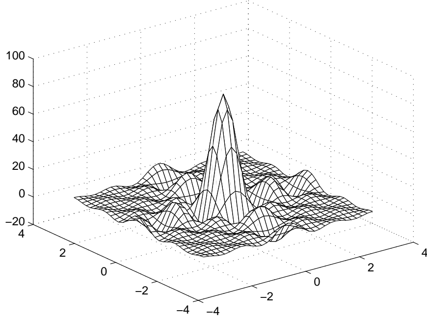
Figure 4.4: The Dirichlet kernel D_n^q with d = 2 , q = \infty , n = 4 .
