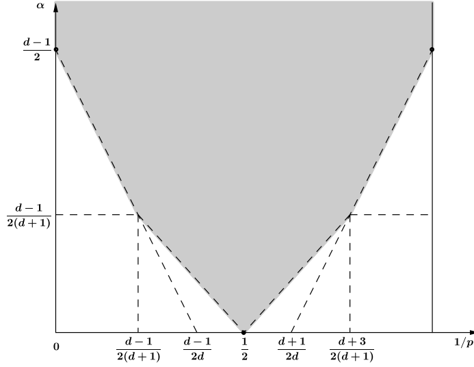
Figure 6.4: Uniform boundedness of \sigma_n^{2,\alpha} when d \geq 3 .
