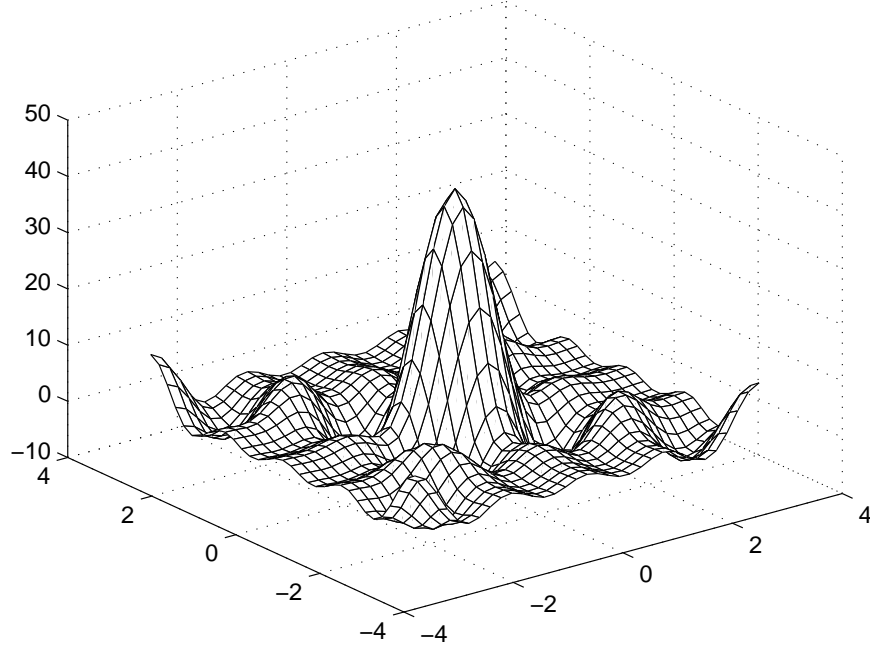
Figure 4.2: The Dirichlet kernel D_n^q with d = 2 , q = 1 , n = 4 .
