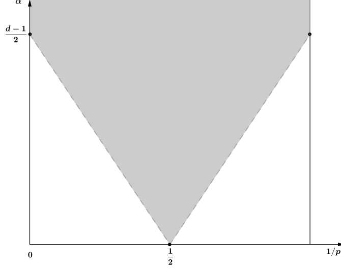
Figure 6.2: Uniform boundedness of \sigma_n^{2,\alpha} when d \geq 3 .
