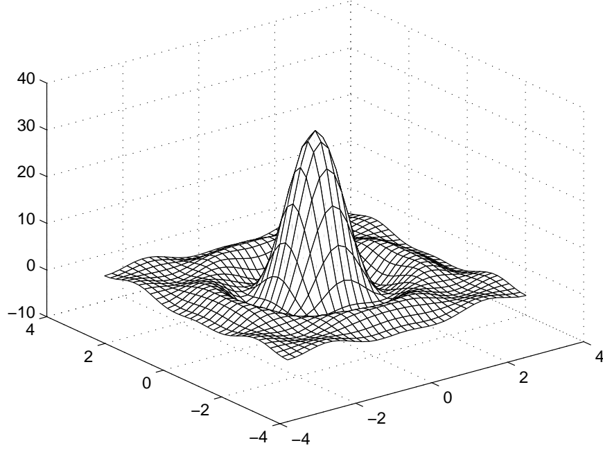
Figure 5.5: The Bochner-Riesz kernel K_n^{q,\alpha} with d = 2 , q = 2 , n = 4 , \alpha = 1/2 , \gamma = 2 .
