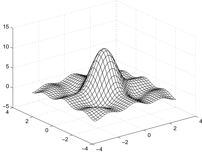
Figure 5.1: The Riesz kernel K_n^{q, \alpha} with d = 2 , q = 1 , n = 4 , \alpha = 1 , \gamma = 1 .
