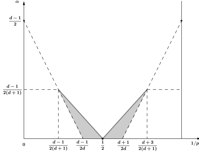
Figure 6.5: Open question of the uniform boundedness of \sigma_n^{2,\alpha} when d \geq 3 .
