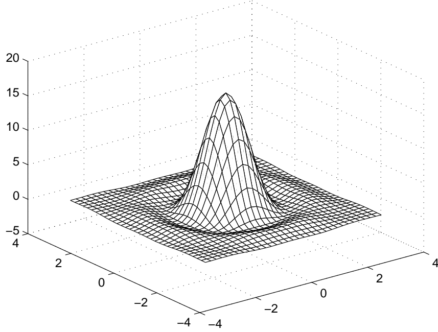
Figure 5.3: The Riesz kernel K_n^{q,\alpha} with d = 2 , q = 2 , n = 4 , \alpha = 1 , \gamma = 1 .
