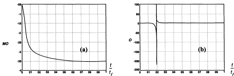
FIGURE 10 Example of temporal variations of \delta_{MO} (a) and \mu_O (b) when O belongs to the space generated by tangents (x_\theta > x_l) but not to (\mathcal{I}_r)
