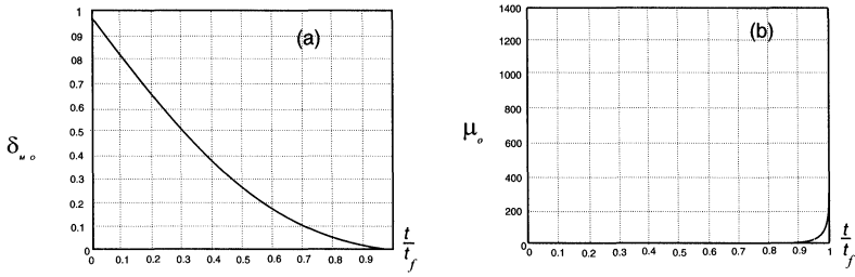
FIGURE 7 Example of temporal variations of \delta_{MO} (a) and \mu_O when O belongs to the straight line ( D_C )
