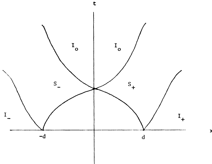
Fig 2.2 : The regions I_a ( a=\pm, 0 ) are constant state regions. The regions S_a^a ( a=\pm ) are the simple wave regions.
