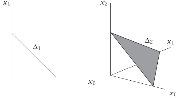
FIGURE 2.1. The standard simplexes \Delta_1 and \Delta_2 .
