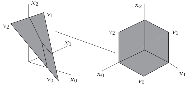
FIGURE 2.2. The 2-simplexes \Delta_2 .
