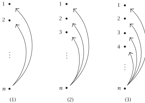
FIGURE 4.2 Tournaments in Propositions 4.2, 4.3, and 4.4.
