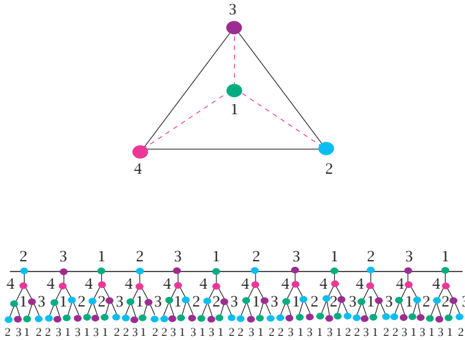
FIGURE 3.1. Tessellation of the 3-regular tree from the complete graph on 4 vertices ( K_4 or the tetrahedron). Obtain the tessellation by choosing a spanning tree in K_4 —the dashed edges. Repeat the spanning tree for each of the infinitely many sheets of the cover. Connections between sheets are forced by the ordering of points on the geodesic labelled with 1, 2, 3 repeated infinitely many times.
