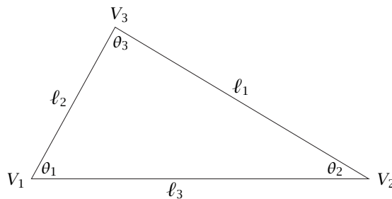
FIGURE 3. \triangle V_1 V_2 V_3 with sides and angles labeled.
