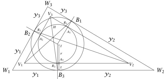
FIGURE 5. The geometry of \triangle V_1V_2V_3 and W_1W_2W_3 .
