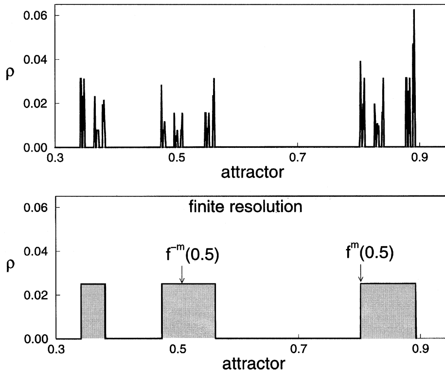
FIGURE 2 Feigenbaum accumulation point: histogram.
