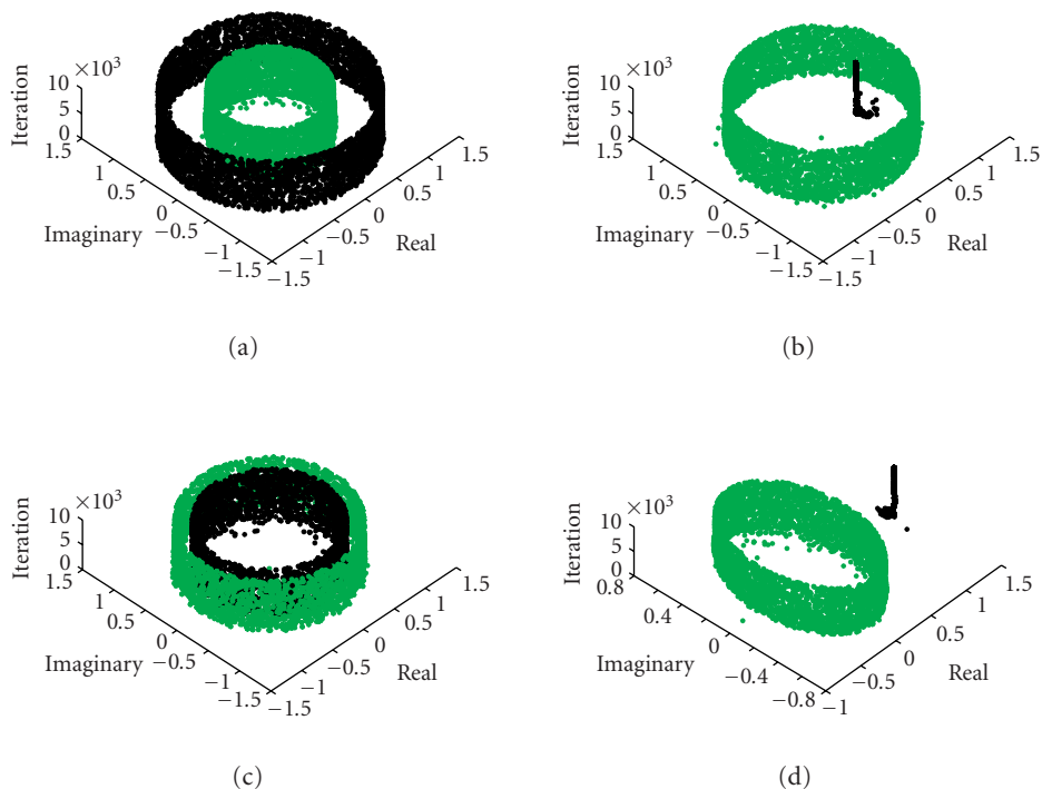
Figure 2.3. Dynamics for random cycles. Shown are the iterates v_n given by (2.1) with (a) a_n = \exp(i\theta_n) , \theta_n \sim U[0, 2\pi] (b) one random strand mod 2, a_{2n+1} = \exp(i\pi/6) , a_{2n} = \exp(i\theta_n) , \theta_n \sim U[0, 2\pi] , (c) one random strand mod 3, a_{3n+1} = a_{3n+2} = \exp(i\pi/6) , a_{3n} = \exp(i\theta_n) , \theta_n \sim U[0, 2\pi] , and (d) one random strand mod 4, a_{4n+1} = a_{4n+2} = a_{4n+3} = \exp(i\pi/6) , a_{4n} = \exp(i\theta_n) , \theta_n \sim U[0, 2\pi] . Odd iterates are light, even iterates are dark.
